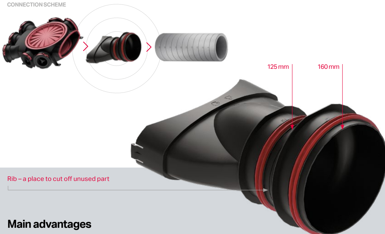
CONNECTION SCHEME
